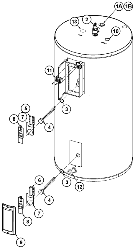
Upright 30, 40, 50, 55, 66, 80, & 120
