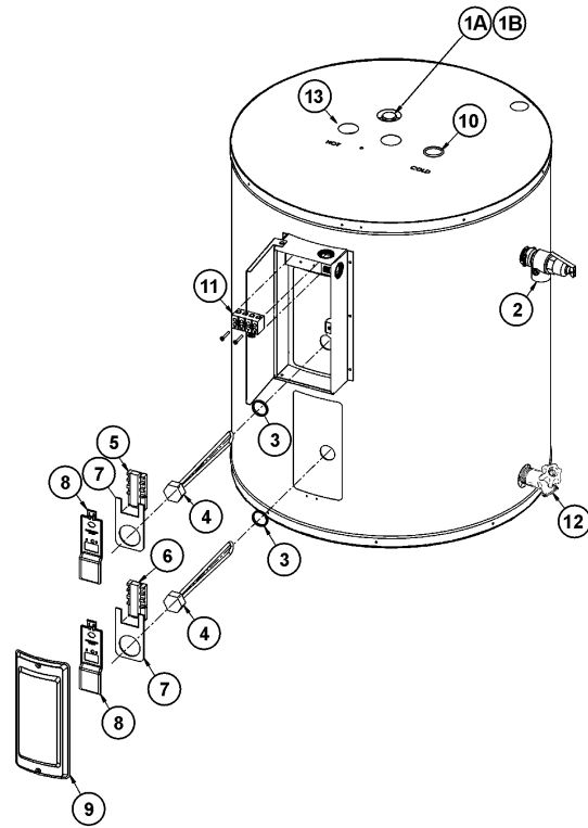
Lowboy 30, 40 & 50
